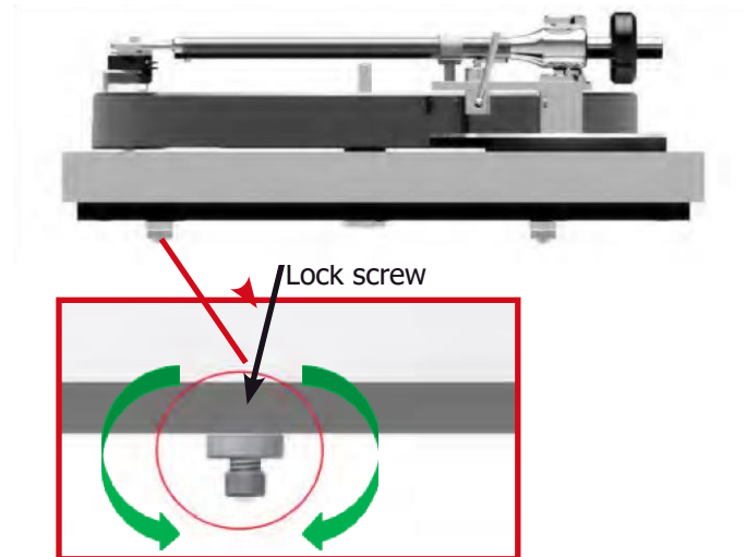
Pic. 7: Adjustment of the turntable feet
