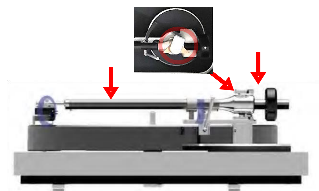
Pic. 5: Remove foam and cardboard piece
